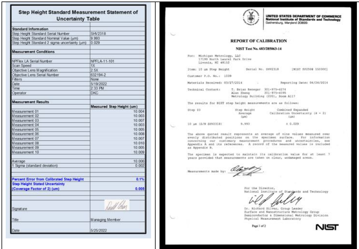
Figure 2. Measurement of NIST Traceable step standard is performed throughout the year for system verification and calibration.
